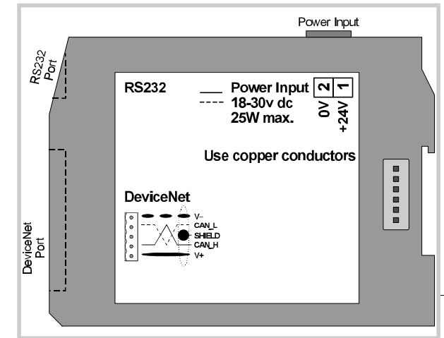
Figure 4 BCM Connectors
